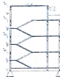
SECTION AT S-S BLOCK-1
